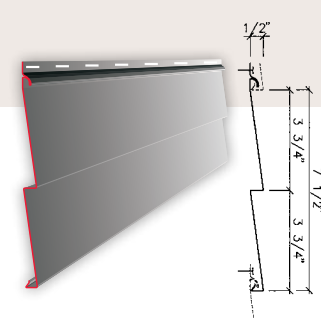
Smooth Horizontal D-4-75
