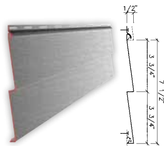
Driftwood Horizontal D-4-75
