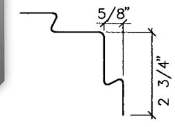
Base Corner Vinyl
