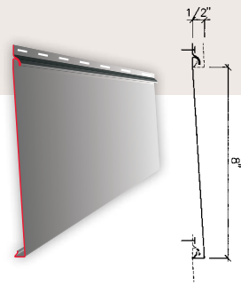
Smooth Horizontal 8"
