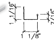
J Channel 1 1/8"
