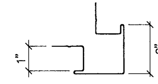
Outside Corner Post
