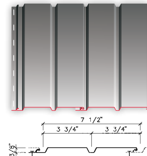
V-Groove Smooth Vertical
