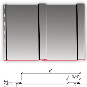
Smooth Vertical 8"
