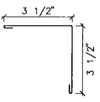
Corner Cap
